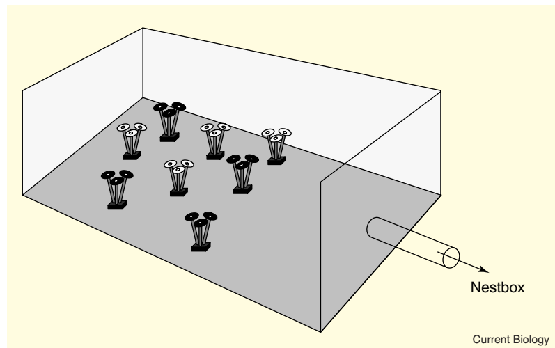
Figure 1. Choice array.
